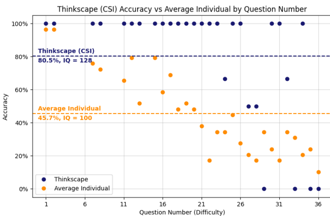
Fig. 5. Performance versus question difficulty for individual test-takers and groups using CSI-powered Thinkscape platform.
