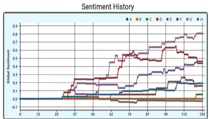
Fig. 8. Real-time Plot of Answer Sentiment vs Time
