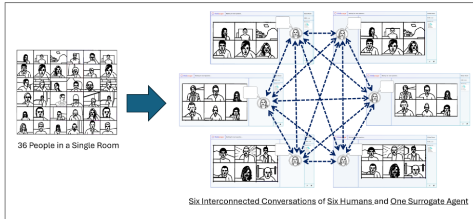
Fig. 6. Example CSI architecture for real-time video-conferencing among 36 people
